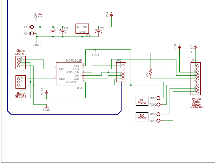
Roll Stand Control Board
