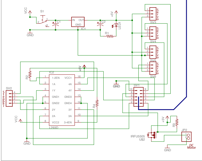
Motor Control Board
